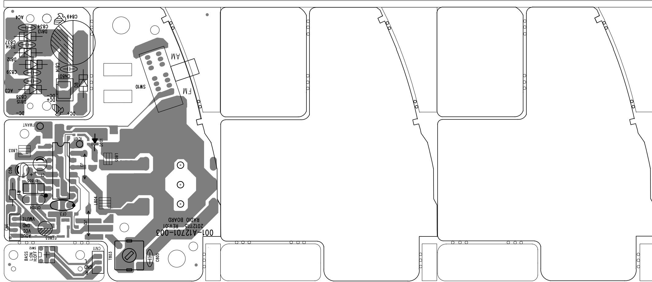
Radio & BBS & Power PCB Layout Bottom Side View
